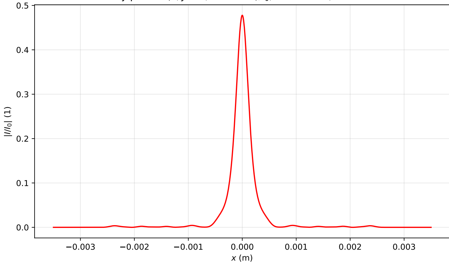
Intensity profile I(x, y = 0, z = 3.344)/I_0 , \text{Pin}=7.0\text{Pcr} , artificial time
